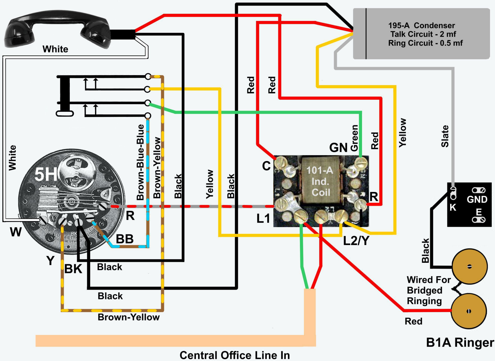
Northern & Western 302 Desk Set Schematic
