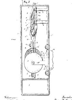
C. R. DAVIS TELEPHONE SIGNAL PAY STATION PATENTED NOV. 21, 1911
