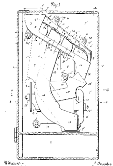
C. R. DAVIS TELEPHONE SIGNAL PAY STATION PATENTED NOV. 21, 1911
