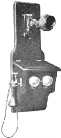
"STYLE 11" WALL TELEPHONE "SERIES 4" FOR BRIDGING."
