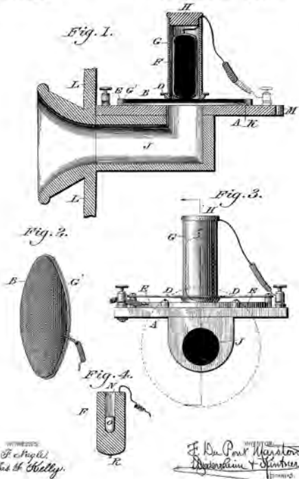
(No Model.) F. DU PONT MARSTON. ELECTRICAL TELEPHONE. No. 380,905. Patented Apr. 10, 1888.
