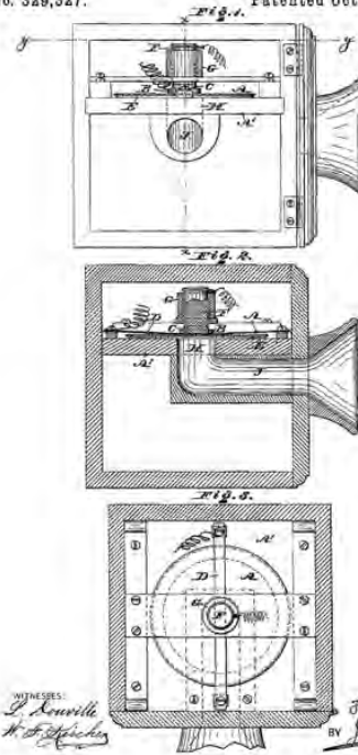
(No Model.) F. DU PONT MARSTON. TELEPHONE TRANSMITTER. No. 329,327. Patented Oct. 27, 1885.
