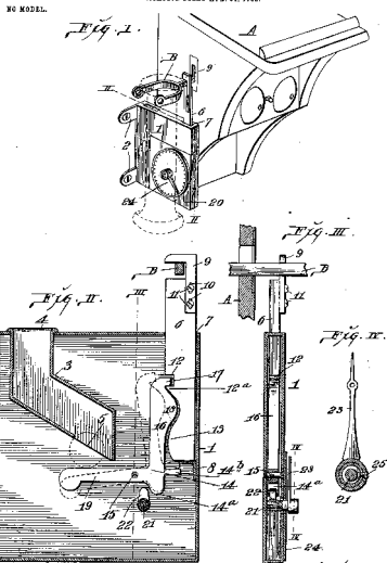
Fig. 2. Stroud Controller.
