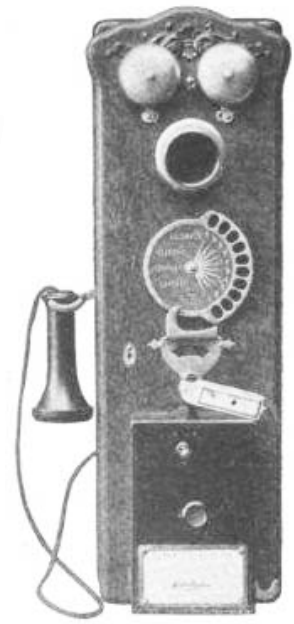
Fig. 2. Automatic Controller.
